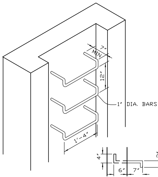
DESIGN FOR PIT RUNGS
