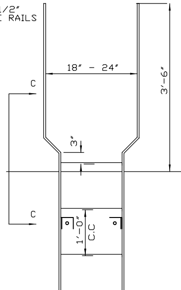
ELEVATION AT PARAPET
