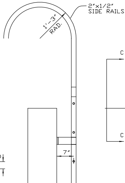
SECTION C-C
